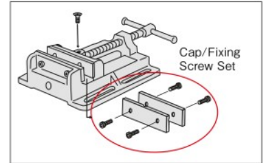
FV100KB (cap/fixing screw set)
