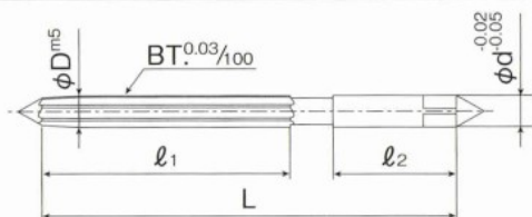
食付き角 1° 1° Chamfer ※図はφ3.0未満の形状です。 Figure is shape of less than φ3.0
